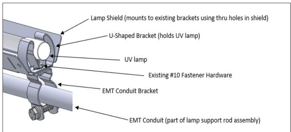
Figure 22: Generic Lamp Shield Installation
