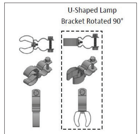
Figure 17: Inverted U-Shaped Lamp Support Bracket - Left Side View (Standard Assembly)
