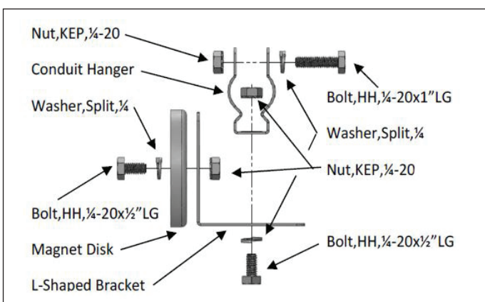
Figure 18: EMT Conduit Bracket Assembly (EXPLODED VIEW)
