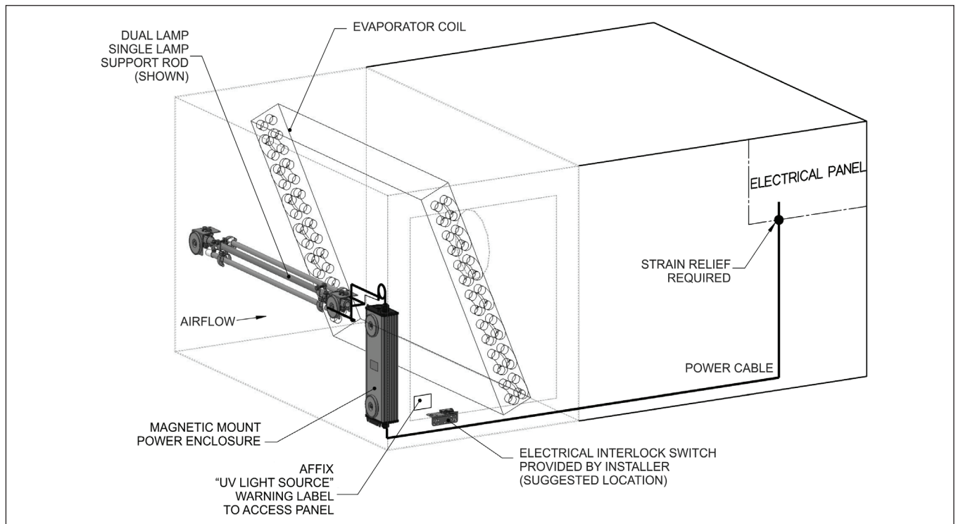
Figure 8: Generic Example of Rooftop HVAC Return Air Side Installation
