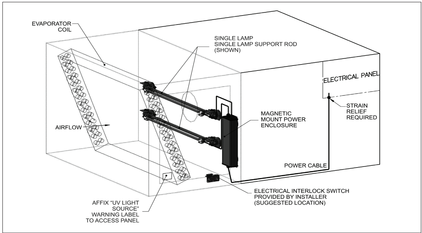
Figure 7: Generic Example of Rooftop HVAC Supply Air Side Installation
