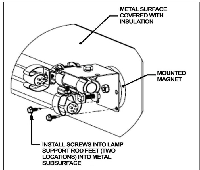
Figure 2B: Alternative Lamp Support Rod Mounting Method using Screws (Screw Mount)
