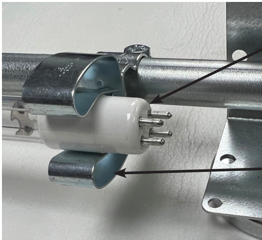
Figure 3A: Correct Lamp Support
