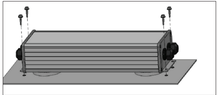
Figure 1B: Alternative Magnetic Mount Power Screw Mounting
