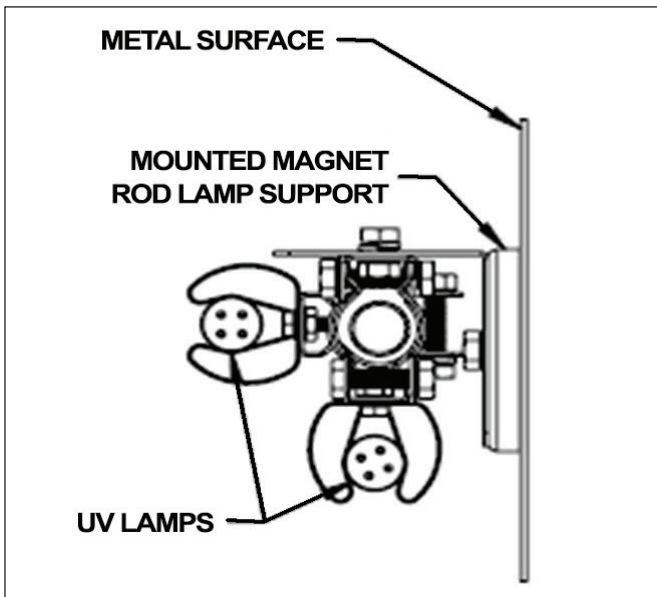
Figure 2A: Lamp Support Rod Standard Mounting (Magnetic Mount)
