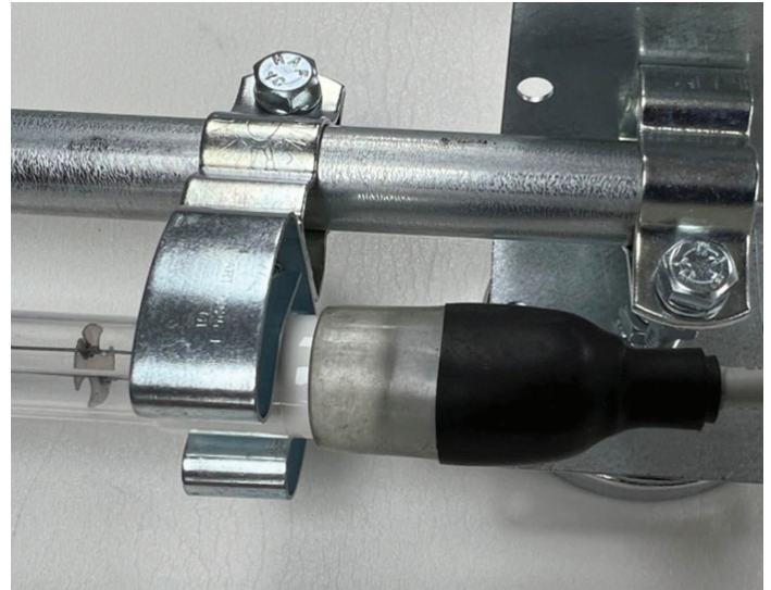
Figure 4B: Proper Cable and Lamp Connection
