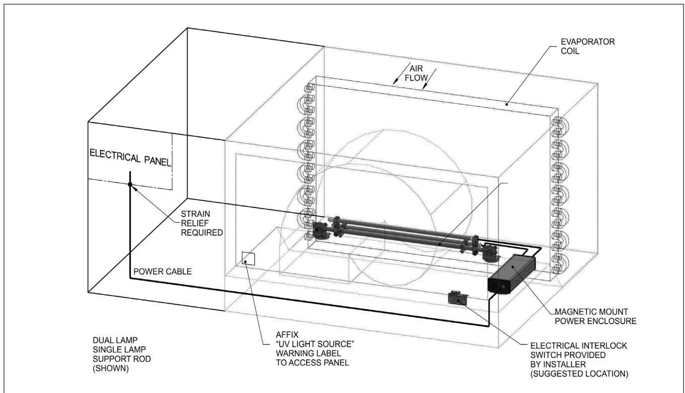
Figure 9: Generic Example of Rooftop HVAC Return Air Side Installation
