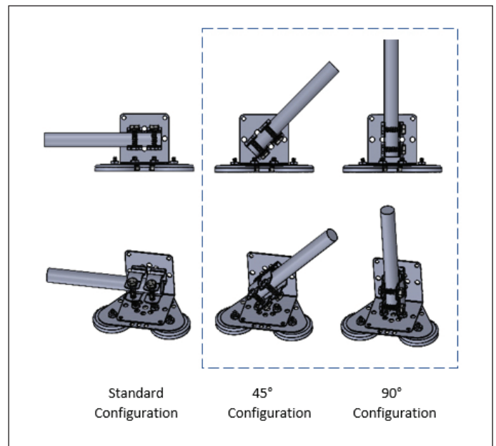
Figure 16: EMT Tri-Foot Magnet Conduit Bracket Assembly for 38 thru 58" UV Lamp Lengths
