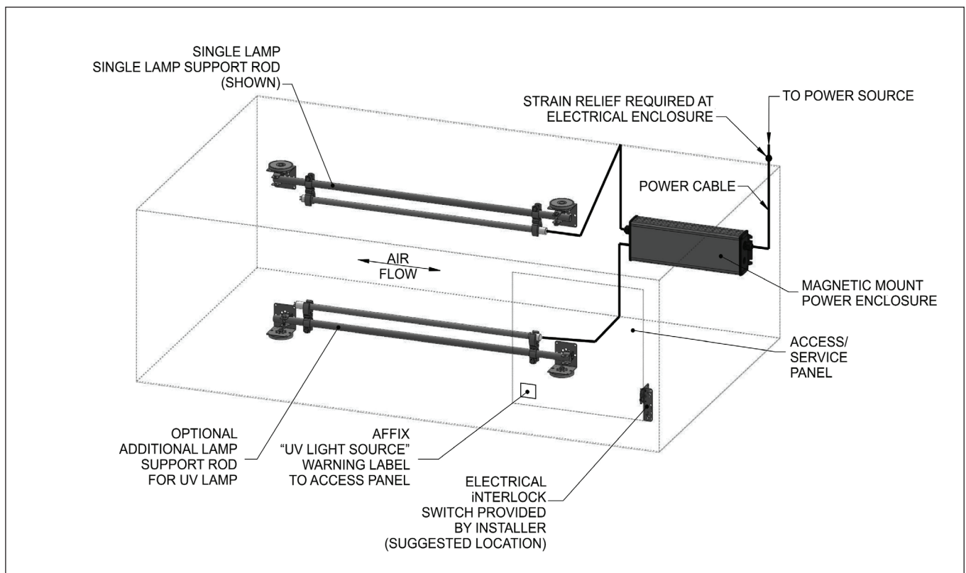
Figure 10: Generic HVAC Ductwork Installation (Horizontal Rod Support)
