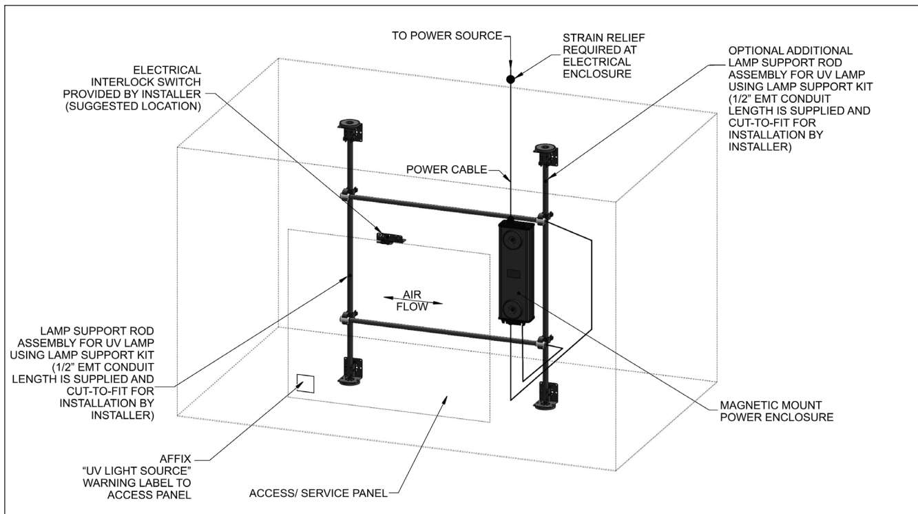
Figure 11: Generic HVAC Ducted Installation (H Style Rod Configuration: Vertical Rod Support with Horizontal Lamp) – Requires Additional Lamp Support Kit with EMT Conduit Mounting Brackets and Inverted U-Shaped Buckets Installed in Alternative Rotated Orientation for Installation
