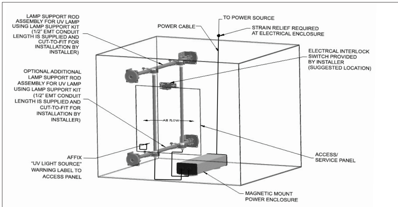
Figure 12: Generic HVAC Ducted Installation (H Style Rod Configuration requires rotated end mounted conduit brackets and rotated U-Shaped lamp support brackets).
