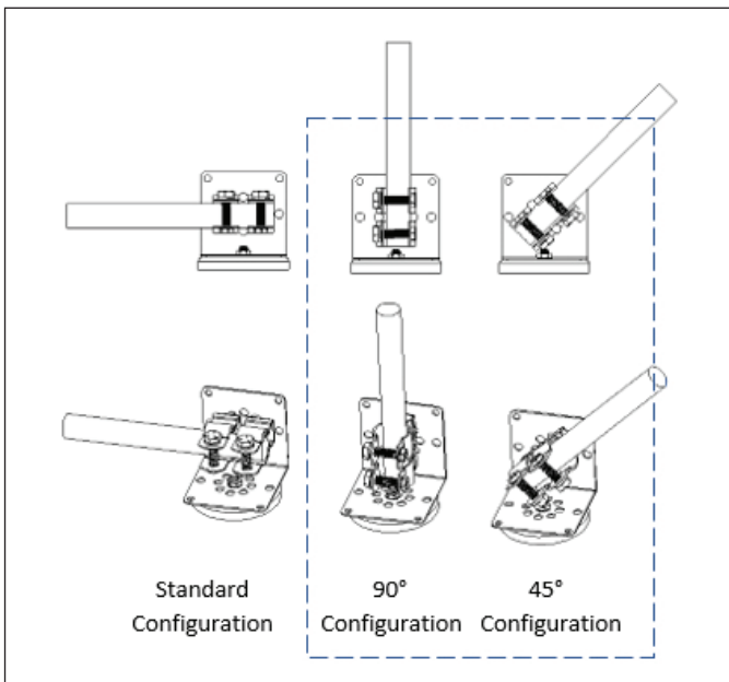
Figure 15: EMT Conduit Bracket Assembly for 18" thru 34" UV Lamp Lengths
