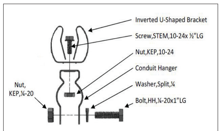
Figure 19: Inverted U-Shaped Lamp Support Bracket (EXPLODED VIEW)
