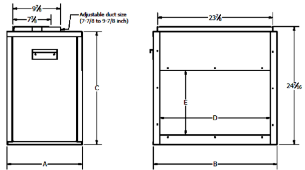
FCRA11-2025 Right Angle Filter Cabinet
