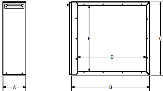
FC8 and FC11 Media Air Cleaner Models
