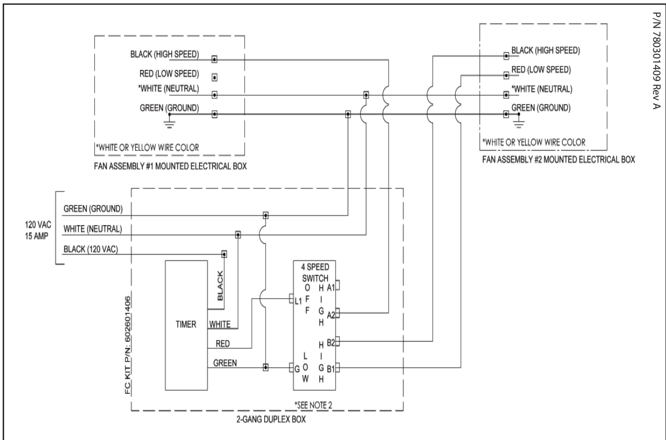
DIAGRAM 2: 4 SPEED CONTROL SWITCH HARDWIRED TO FAN
