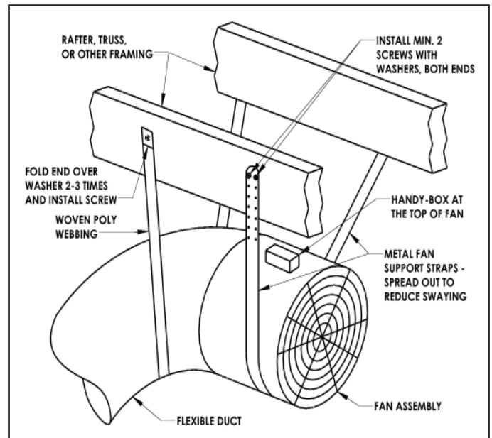
FIGURE 3: FAN & DUCT STRAPS DETAIL
