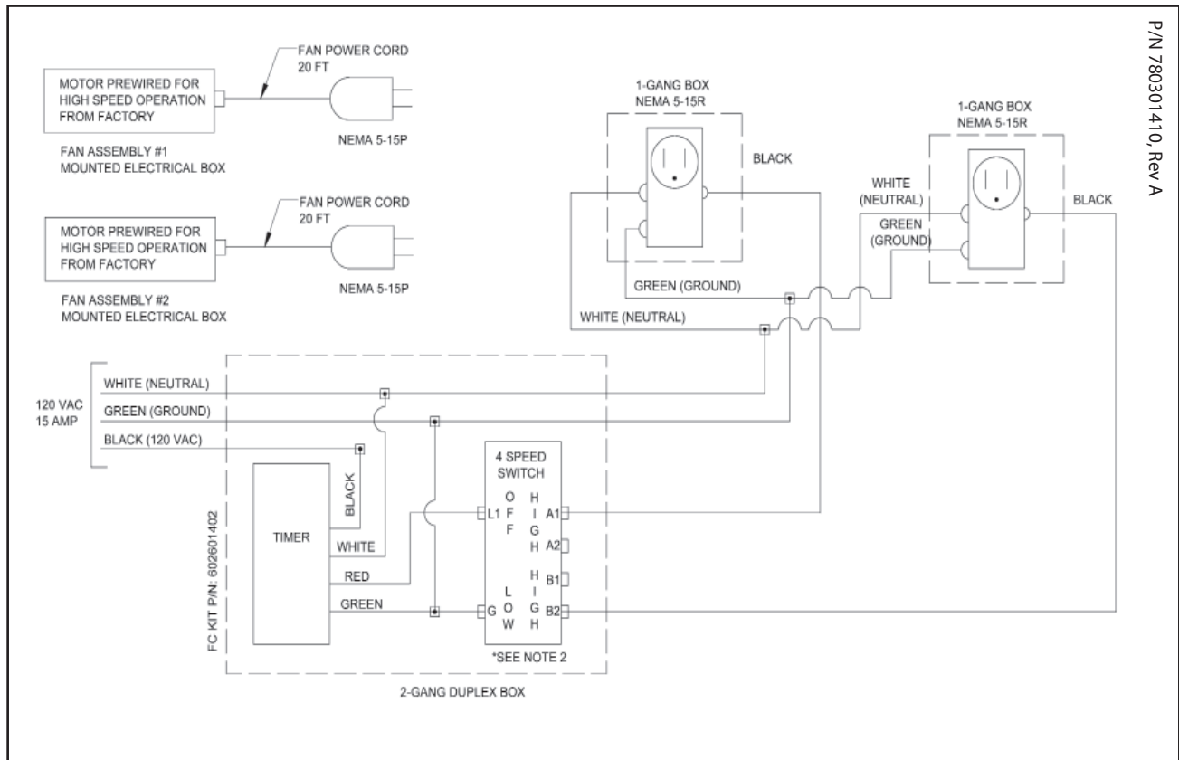
DIAGRAM 1: 4 SPEED CONTROL SWITCH USING FAN POWER CORD
