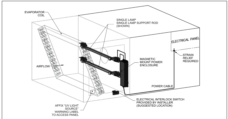
Generic Example of Rooftop HVAC Supply Air Side Installation
