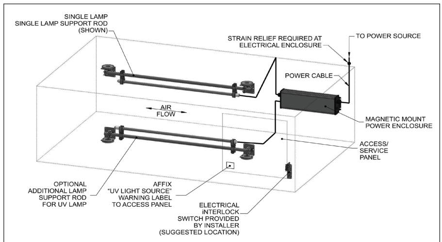
Generic HVAC Ductwork Installation (Horizontal Rod Support)
