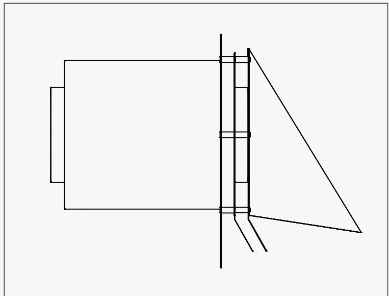
Figure 1 - Typical Side Wall Vent Hood
