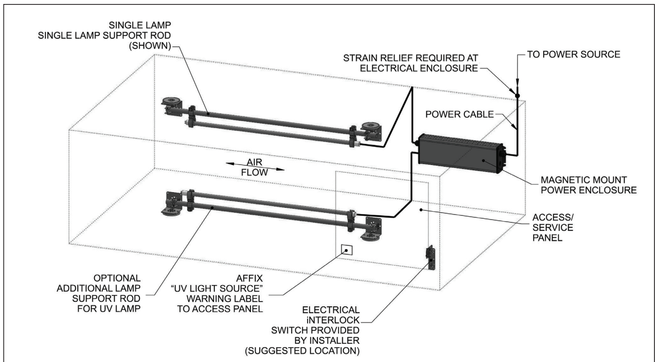
Figure 10: Generic HVAC Ductwork Installation (Horizontal Rod Support)
