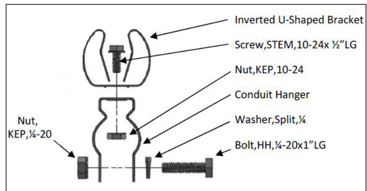
Figure 19: Inverted U-Shaped Lamp Support Bracket (Exploded View)
