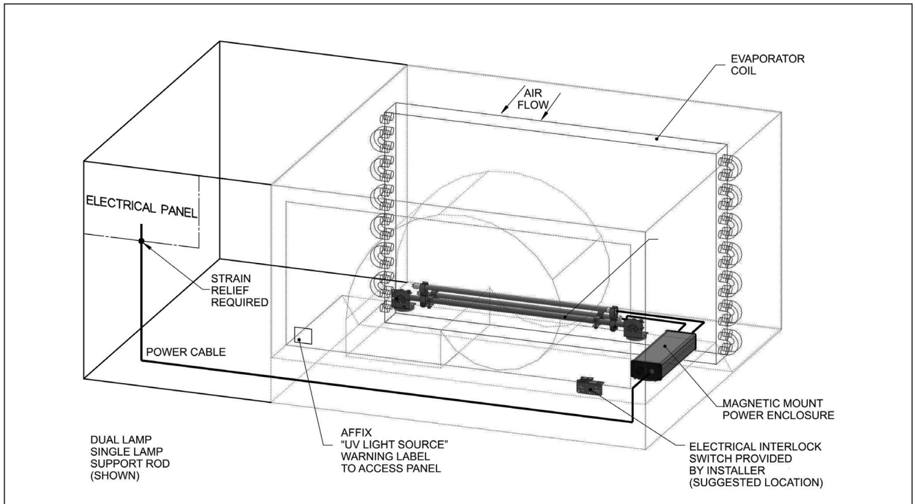
Figure 9: Generic Example of Rooftop HVAC Return Air Side Installation
