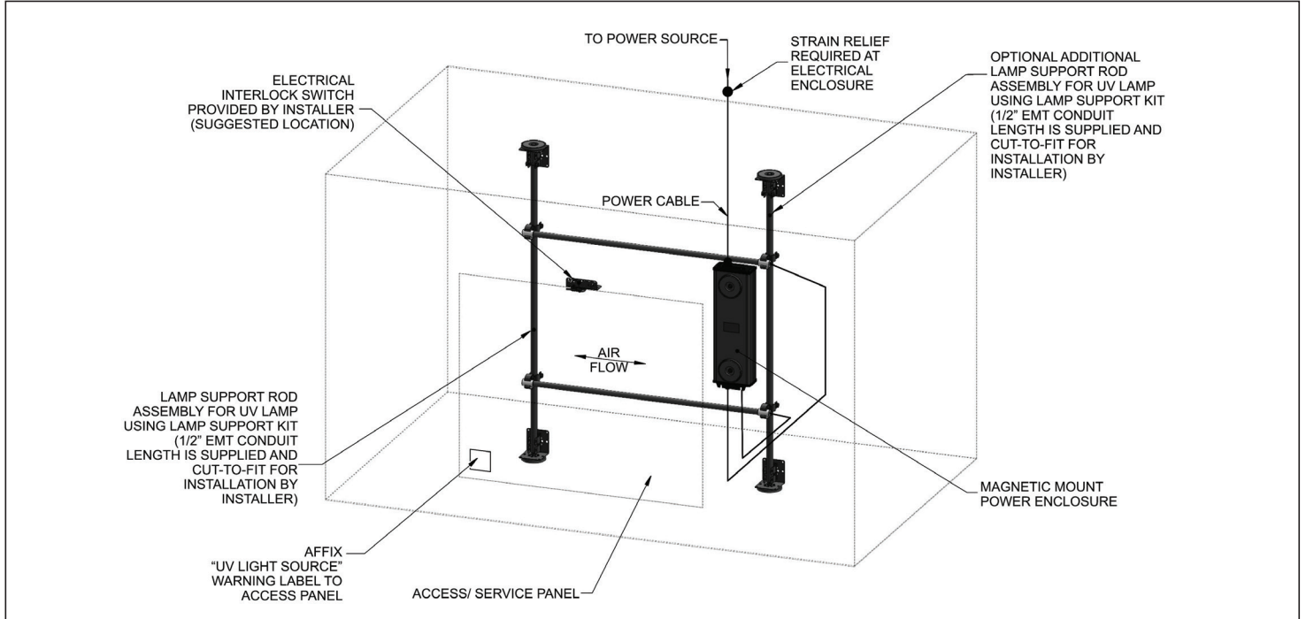
Figure 11: Generic HVAC Ducted Installation (H Style Configuration: Vertical Rod Support with Horizontal Lamp)- Requires Additional Lamp Support Kit with EMT Conduit Mounting Brackets and Inverted U-Shaped Brackets Installed in Alternative Rotated Orientation for Installation.
