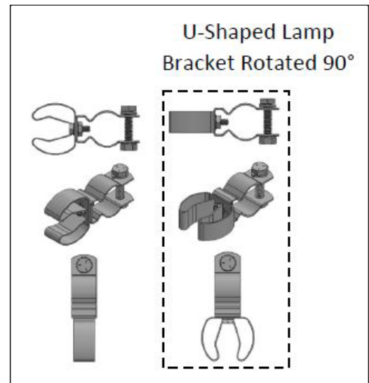
Figure 17: Inverted U-Shaped Lamp Support Bracket - Left Side View (Standard Assembly)
