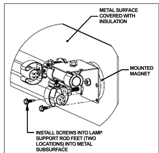
Figure 2B Alternative Lamp Support Rod Mounting Method using screws (Screw Mount)
