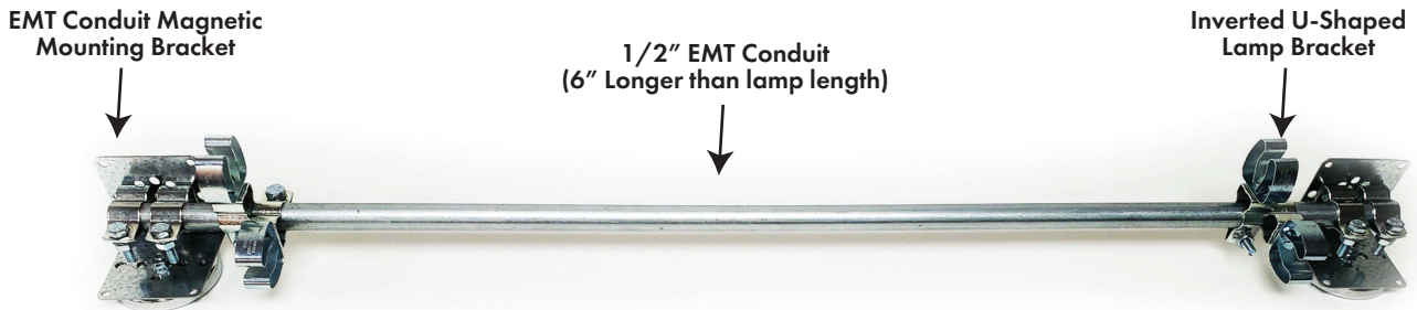
Figure 14: Dual Lamp Support Rod Assembly for Dual Lamp Models (Optional)
