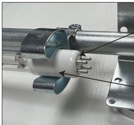
Figure 3A Correct Lamp Support
