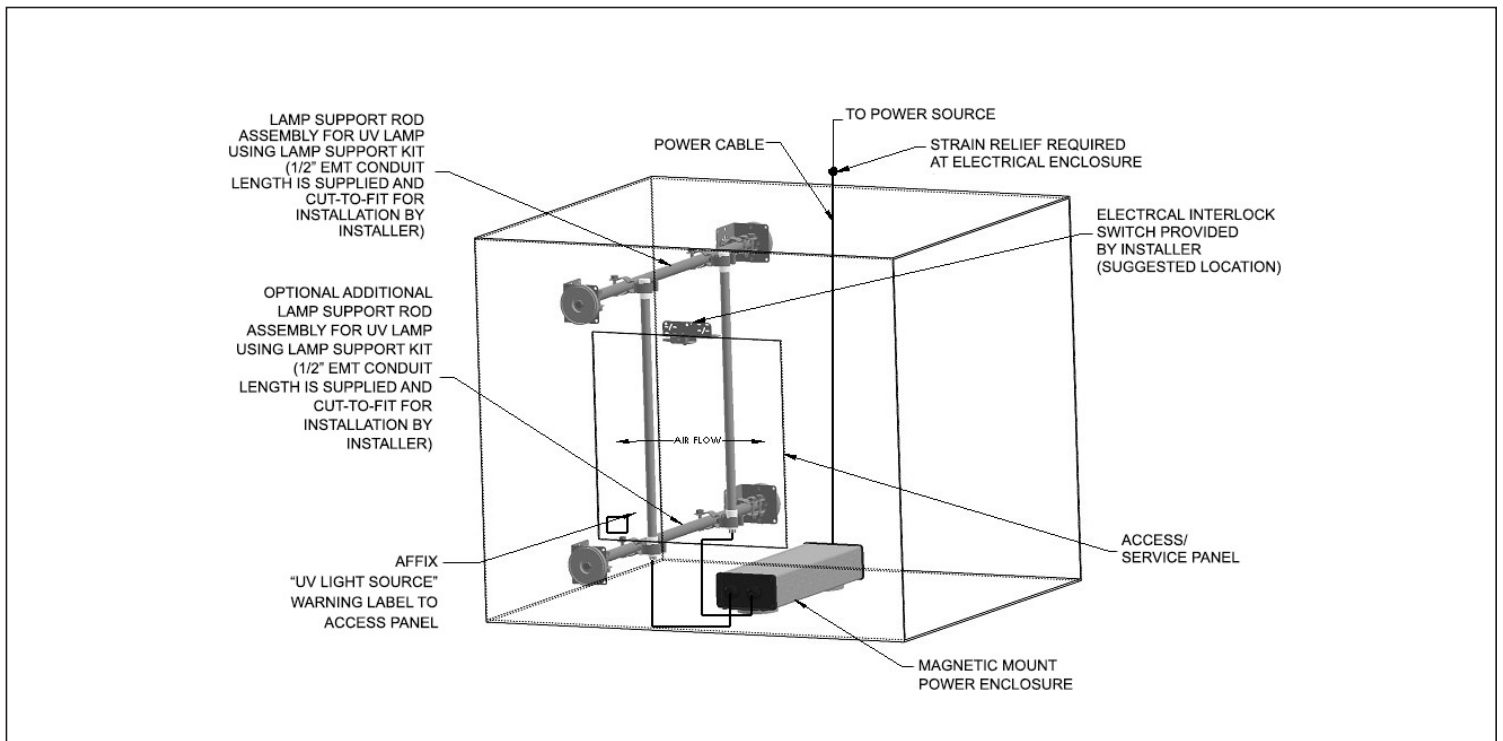
Figure 12: Generic HVAC Ducted Installation (H Style Rod Configuration requires rotated end mounted conduit brackets and rotated U-Shaped lamp support brackets).
