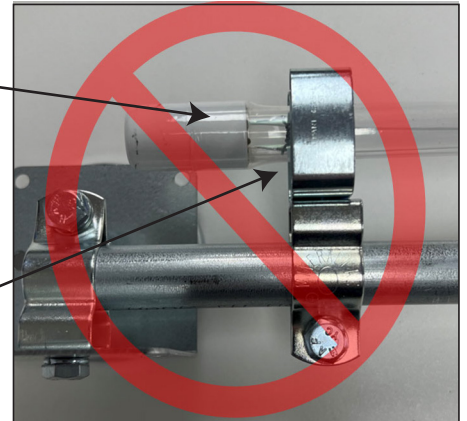
Figure 3B Incorrect Lamp Support
