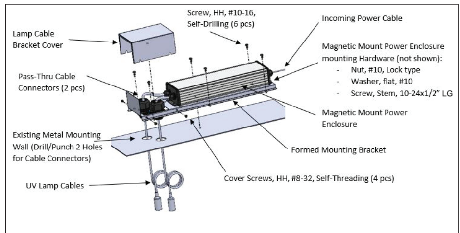
Figure 21: Outdoor Mounting Kit
