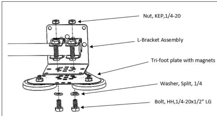
Figure 20: EMT Tri-Foot Partial Assembly (Exploded View)
