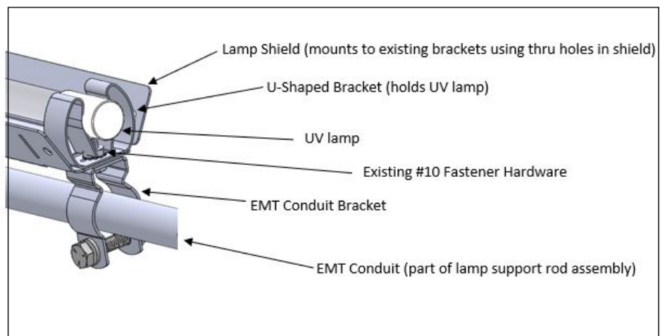
Figure 22: Generic Lamp Shield Installation
