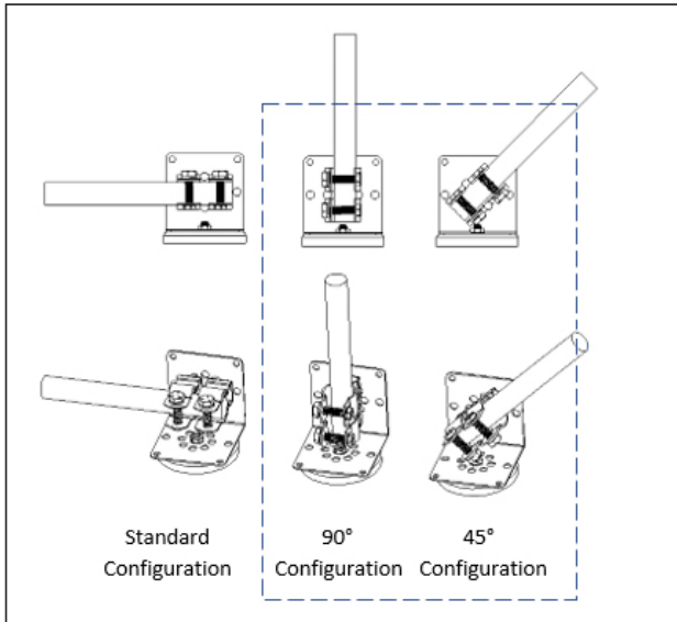
Figure 15: EMT Conduit Bracket Assembly for 18" thru 34" UV Lamp Lengths
