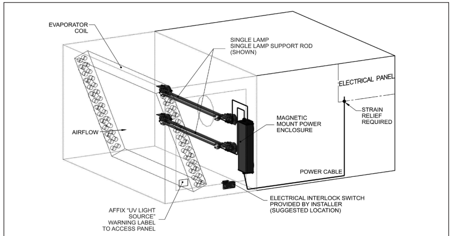
Generic Example of Rooftop HVAC Supply Air Side
