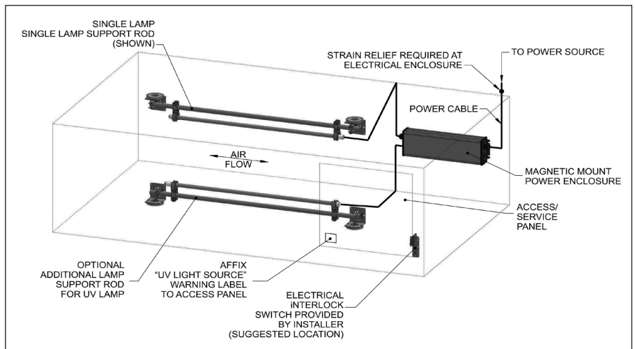
Generic HVAC Ductwork Installation (Horizontal)
